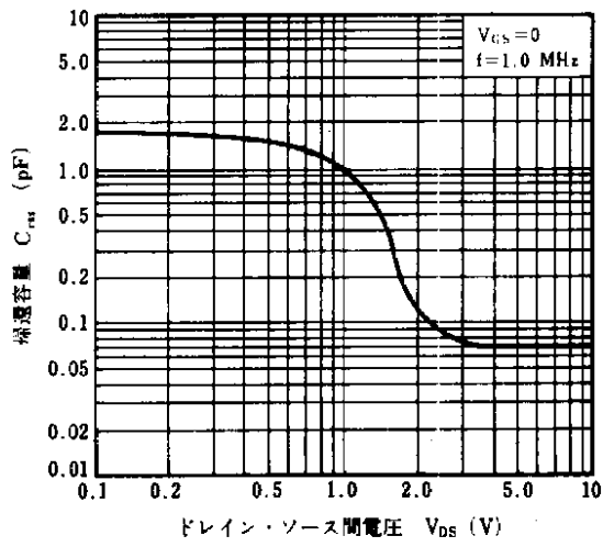
FEEDBACK CAPACITANCE vs. DRAIN TO SOURCE VOLTAGE
