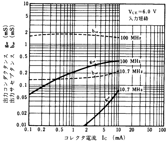
OUTPUT ADMITTANCE ( y_{oe} ) vs. COLLECTOR CURRENT
