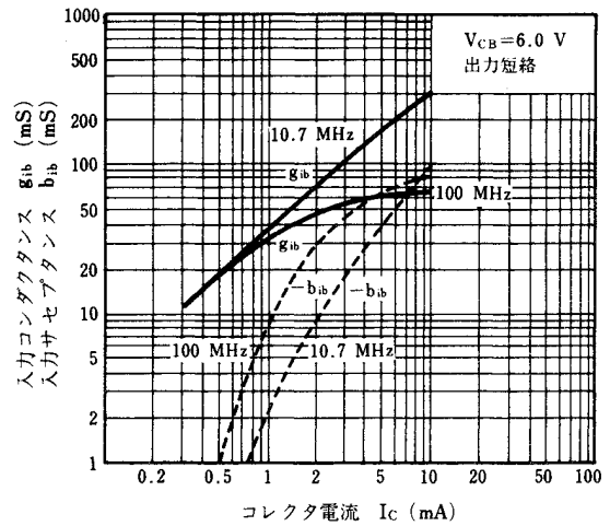
INPUT ADMITTANCE ( y_{ib} ) vs. COLLECTOR CURRENT
