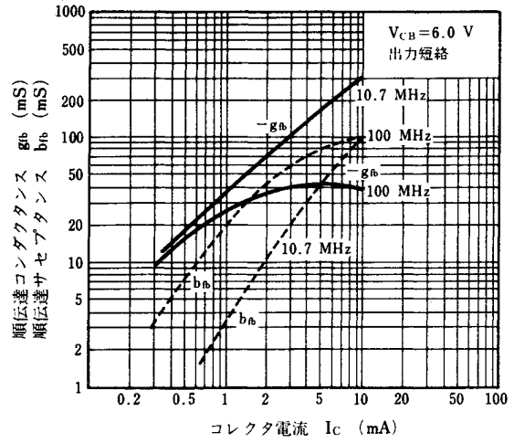
FORWARD TRANSFER ADMITTANCE ( y_{fb} ) vs. COLLECTOR CURRENT
