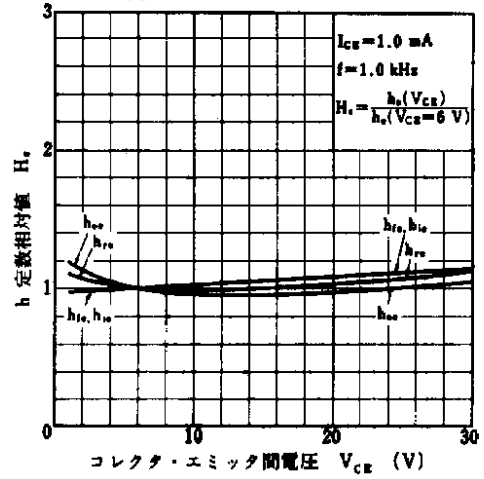
NORMALIZED h-PARAMETER vs. COLLECTOR TO EMITTER VOLTAGE
